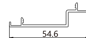
YF-5784 KG/M:0.291 Door Frame Cover
