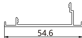
YF-5785 KG/M:0.290 Door Frame Bottom Cover
