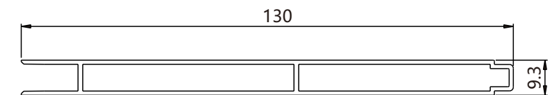
XYX8342B KG/M:0.855 Aluminium Side Panel
