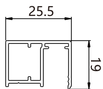
YF-5787 KG/M:0.292 Interior Casing
