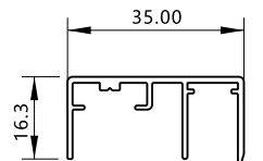
YF-5782 KG/M:0.298 Interior Casing
