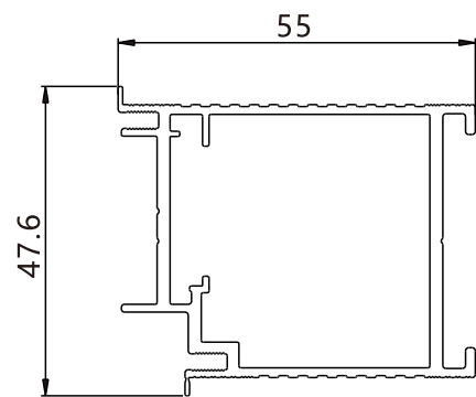
YF-5783 KG/M:0.940 Door Frame
