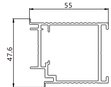
YF-5783 KG/M:0.940 Door Frame
