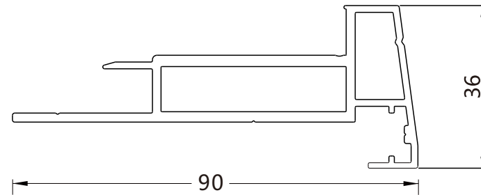
YF-5786 KG/M:1.260 Exterior Casing
