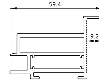
YF-5781 KG/M:1.27 Exterior Casing
