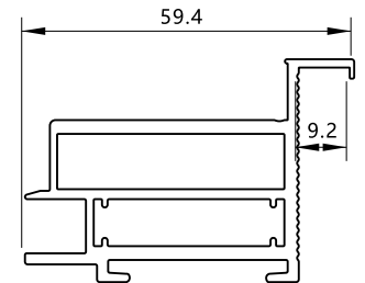
YF-5781 KG/M:1.27 Exterior Casing
