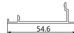
YF-5785 KG/M:0.290 Door Frame Bottom Cover
