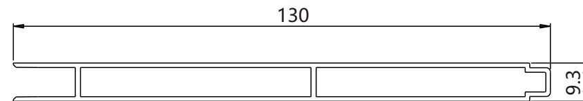
XYX8342B KG/M:0.855 Aluminium Side Panel
