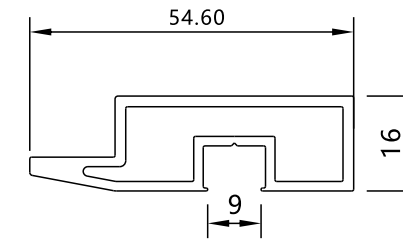
YF-5788 KG/M:0.695 Door Frame
