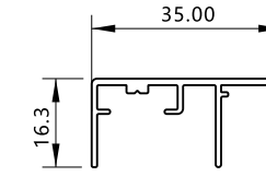
YF-5782 KG/M:0.298 Interior Casing
